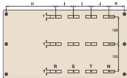
밑면도 (Bottom View)
