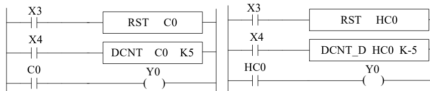
Common count up counter
